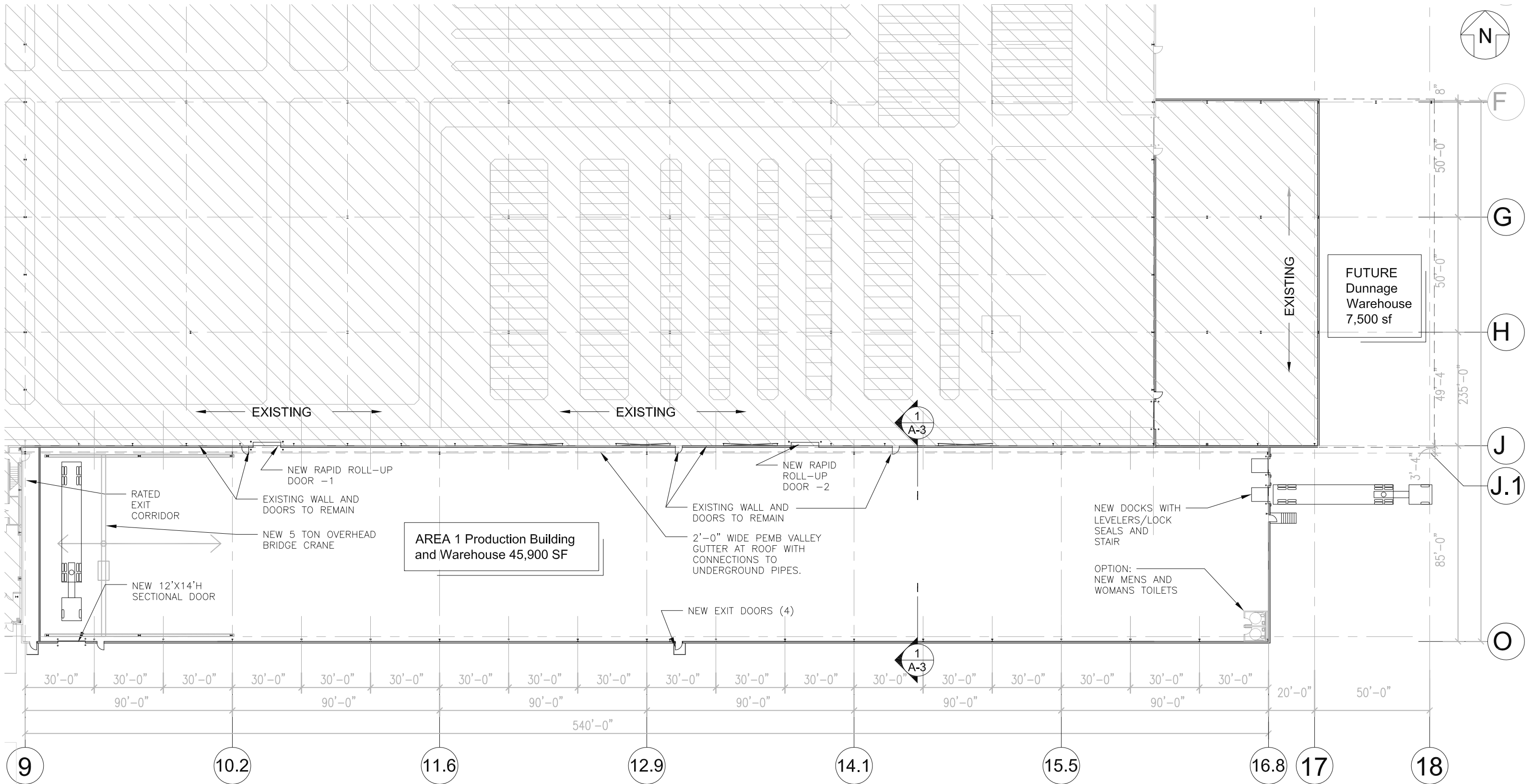
1 Partial Floor Plan 1/40" = 1'-0"
