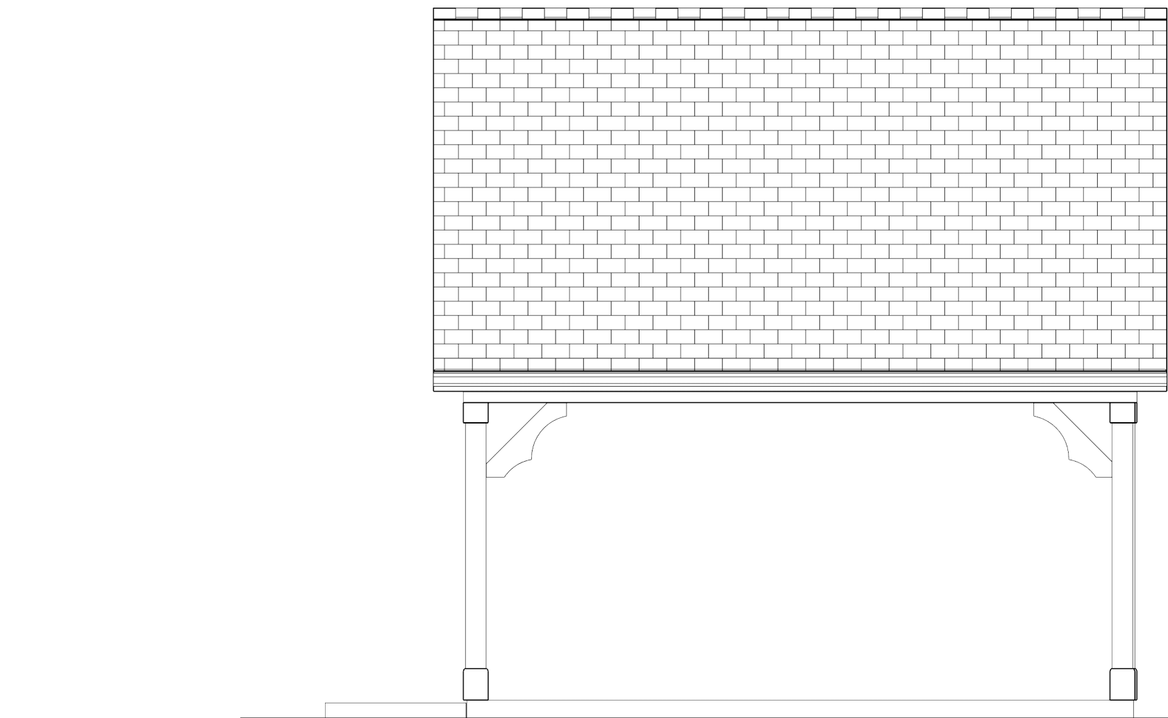
EAST ELEVATION SCALE: 1/4"=1'
