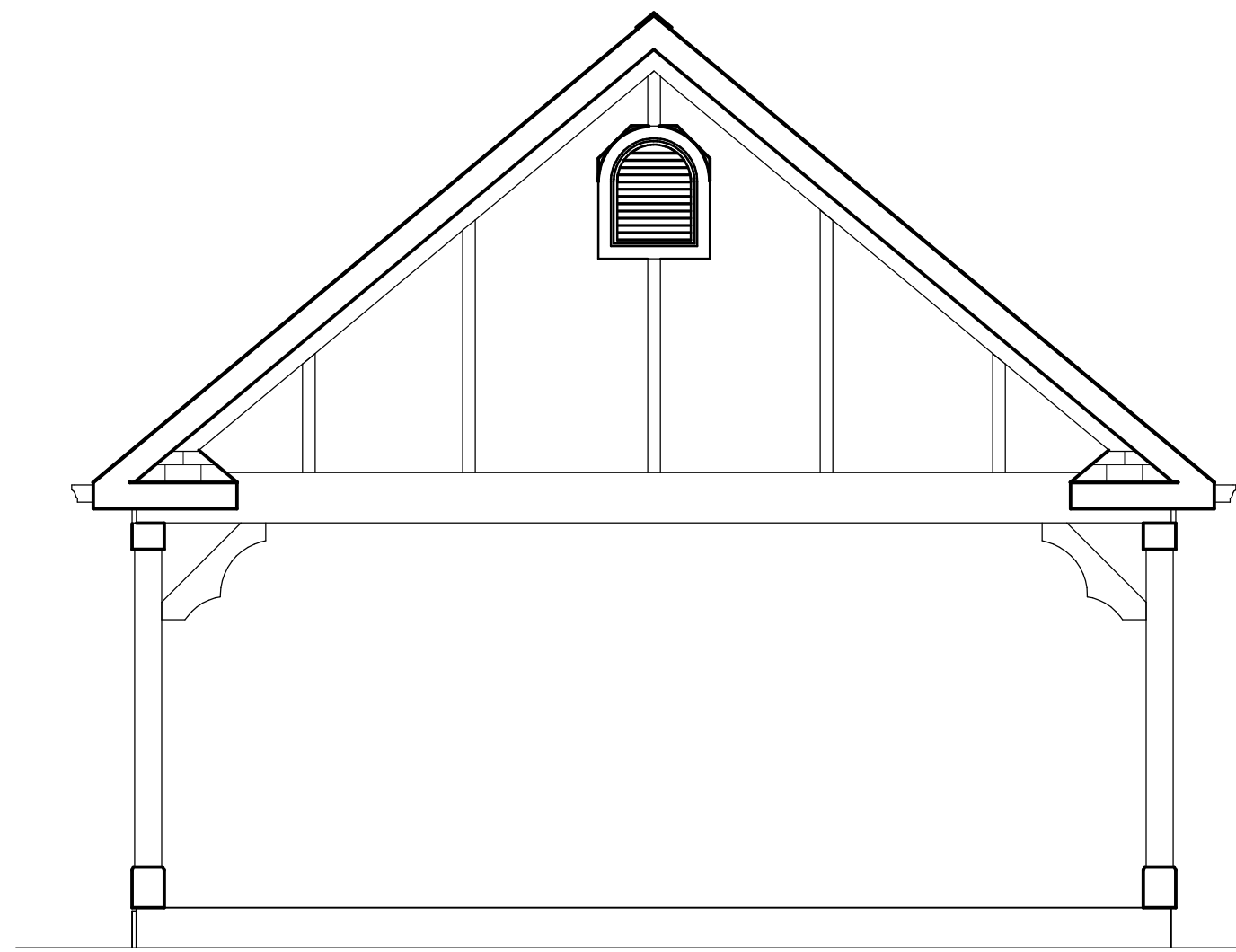
SOUTH ELEVATION SCALE: 1/4"=1'
