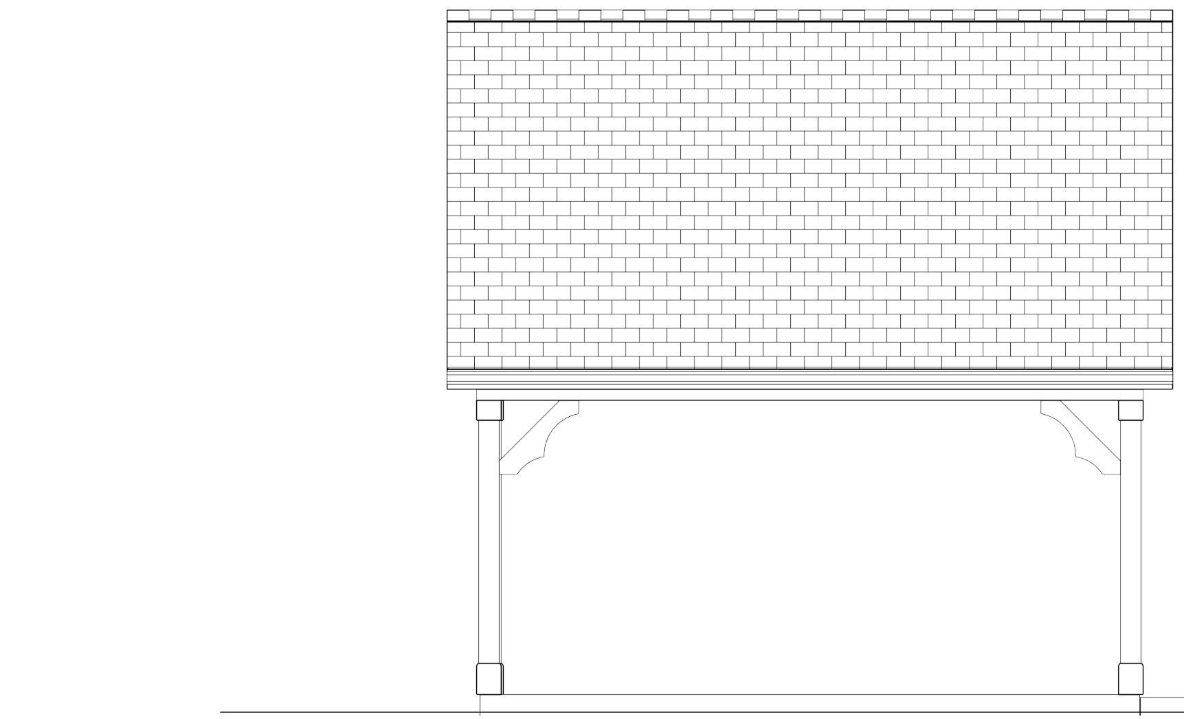
WEST ELEVATION SCALE: 1/4"=1'
